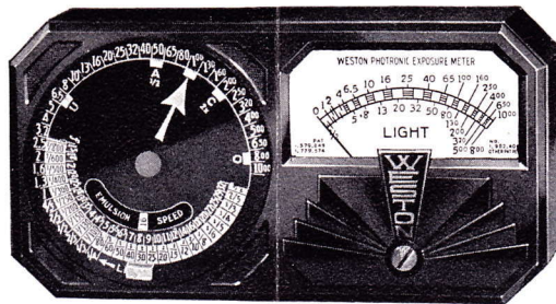
MODEL 650 EXPOSURE METER
